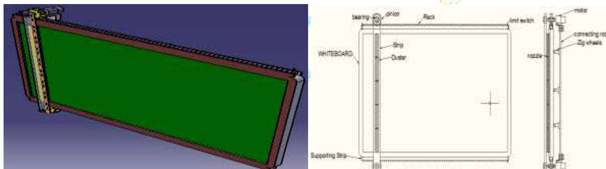
Figure 3: 3D, Side and Front View of Automatic Board Cleaning System
